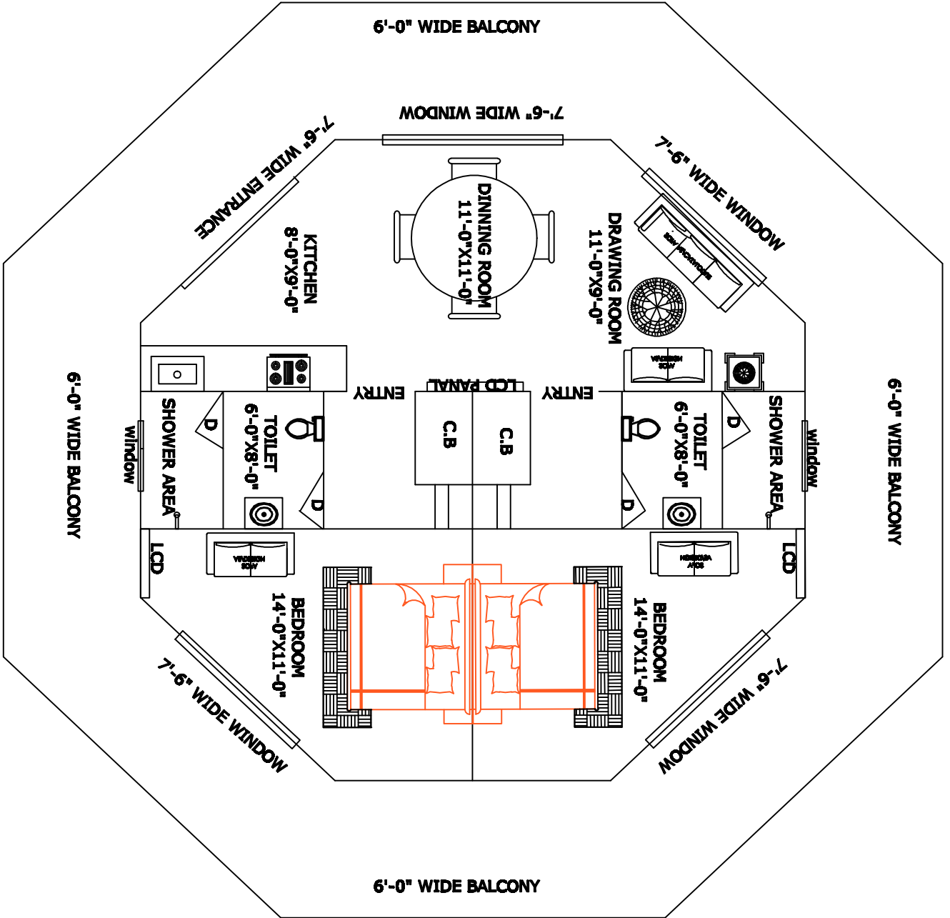
2BHK LAYOUT PLAN
